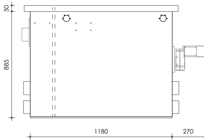
Right-side view
